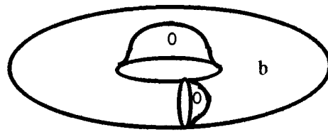
FIGURE 2.7. Identification A yields the equation \mathbf{b} = \mathbf{a} + \mathbf{b} \Rightarrow \mathbf{a} = 0 . Identification B yields the equation \mathbf{b} = \mathbf{b} + \mathbf{c} \Rightarrow \mathbf{c} = 0 . So the weight systems on W are (where \mathbf{b} is a nonnegative integer)
