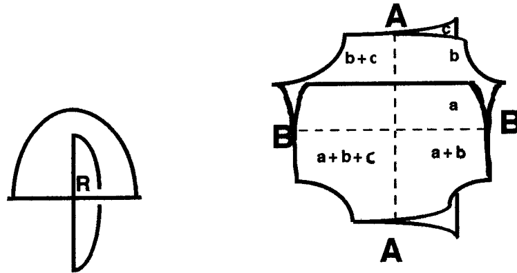
FIGURE 2.7. Identification A yields the equation \mathbf{b} = \mathbf{a} + \mathbf{b} \Rightarrow \mathbf{a} = 0 . Identification B yields the equation \mathbf{b} = \mathbf{b} + \mathbf{c} \Rightarrow \mathbf{c} = 0 . So the weight systems on W are (where \mathbf{b} is a nonnegative integer)
