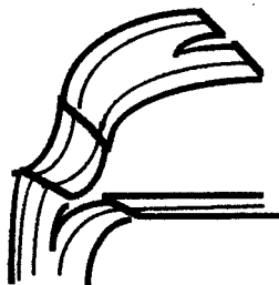
FIGURE 2.5. An example of how a foliation of N(W_\varepsilon) appears locally.
